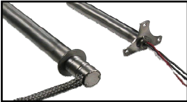
Flanges: Standard flange material is stainless steel. Flanges can be round, irregularly shaped, or even as simple as a bead of weld. Contact Jobco for standard and non-standard flange configurations.
